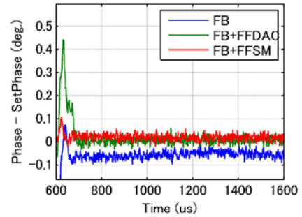
Figure 4: Comparison of amplitude and phase measured at flat-top region. Under FB + FFDAC or FB + FFSM condition, stability at 700\sim 1600\ \mu\text{s} is 0.007\% rms and 0.015^\circ rms.
