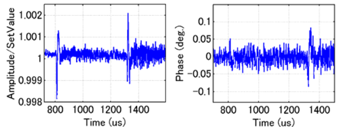
Figure 8: Flat-top stability around quasi-beam injection in FB + FF table(including beam compensation) operation with timing adjustment.
