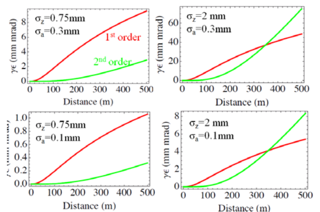
Figure 1: Projected emittance.
