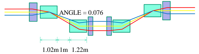
Figure 6: Bunch flip at SY2.
