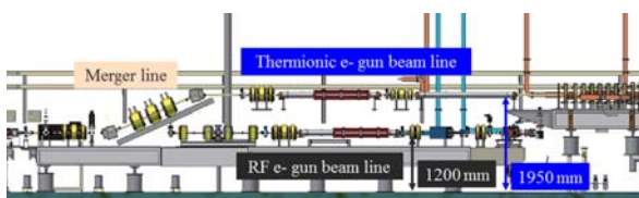
Figure 7: Layout of the new thermionic electron gun beamline. The existing beam line is kept for the rf electron gun. The bunching section of thermionic electron gun is constructed at the beam line height of 1950 mm from the floor though the height of original beam line is 1200 mm from the floor.
