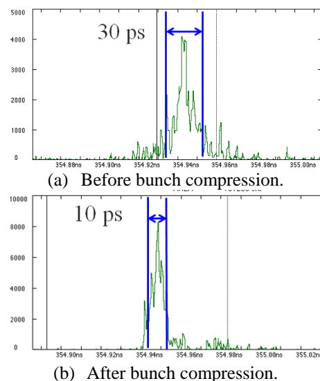
Figure 3: Bunch length measured by a streak camera before (a) and after (b) bunch compression at the chicane of injector section.
