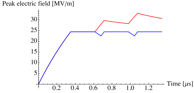
Figure 4: Accelerator peak gradient on standing wave L-band RF cavity. Blue line shows the constant gradient at beam acceleration. This gradient is generated by the input power Fig. 5. The other gradient shown by red line is generated by constant input power to RF cavity.
