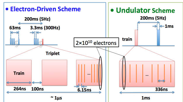
Figure 2: Multi-bunch structures on the electron-driven scheme before DR (left) and on the undulator scheme (right).
