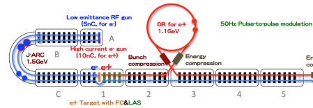
Figure 1: Schematic layout of the SuperKEKB injector linac.
