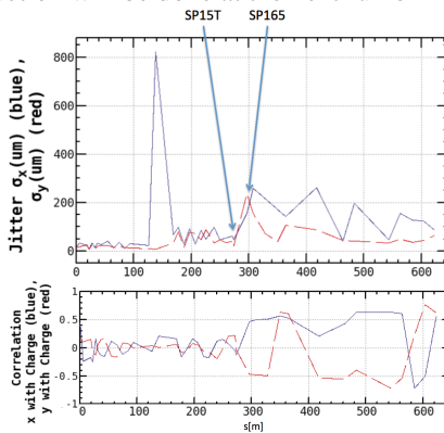
Figure 6: Beam position jitter in the linac and correlations between beam positions and charge. Blue and red show horizontal and vertical correlations, respectively.
