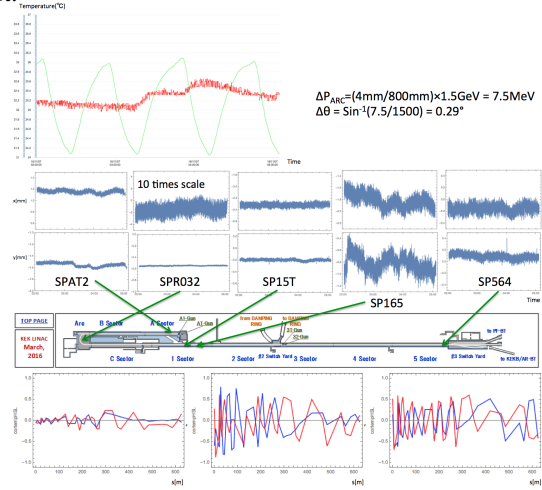
Figure 7: Temperature around electron gun, beam position jitter, and these correlations.
