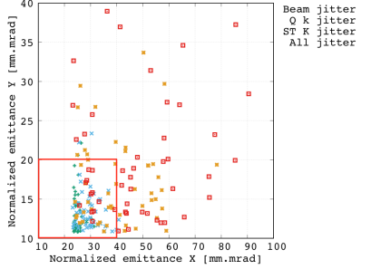
Figure 5: Emittance growth by beam, quadrupole, and steering jitters.
