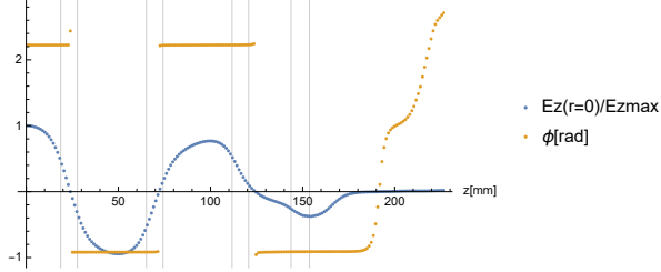
Figure 8: The accelerating field E_z(z, r = 0) calculated by numerical simulation.
