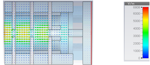
Figure 6: The contour plot of the tangential component of the electric field calculated using CST.
