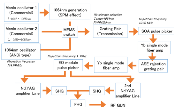
Figure 1: Layout of Laser system.
