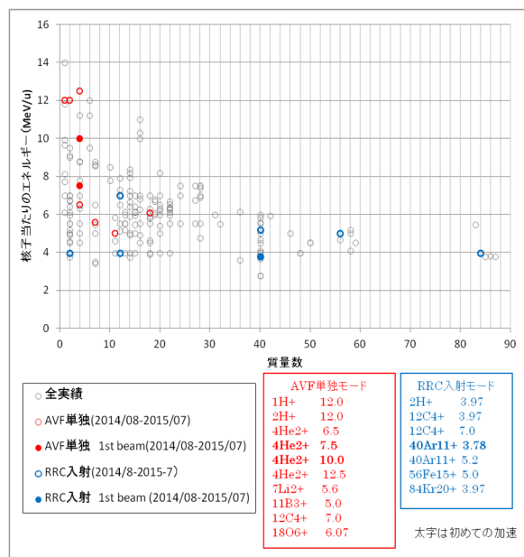
Figure 1: Energy-Mass map of AVF.
