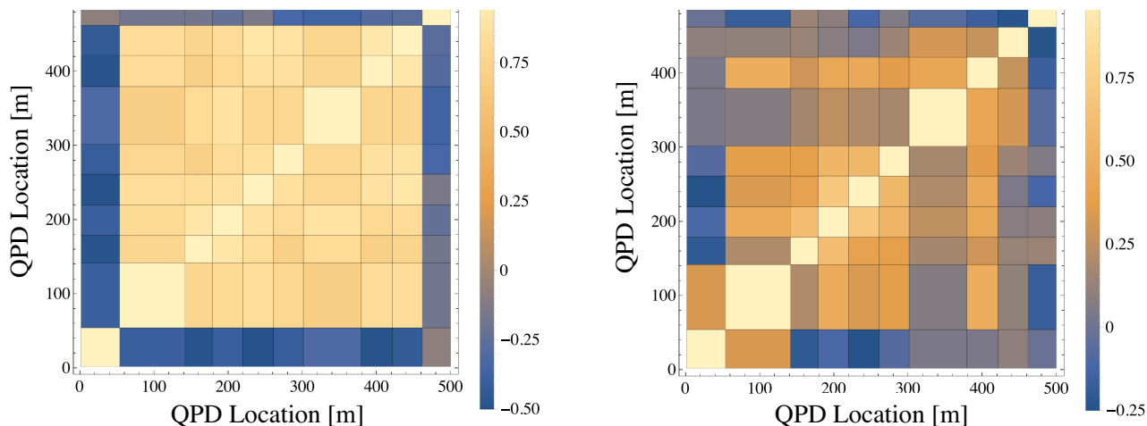
Figure 4: Intensity distributions in the cross-correlation function between all the QPDs in the displacement vector measurements of the accelerator units along the C5 straight section obtained at (a) Feb.15.2016, 0:00 am and (b) Feb.27.2016, 8:00 am. It should be noted that any correlation functions on a straight line tilted at 45 degree passing through the axis origin are defined as a self-correlation function, that is, \hat{R}_0=1 .
