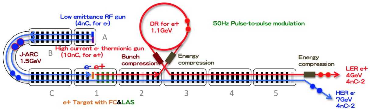
Figure 1: Schematic layout of the SuperKEKB injector linac.
