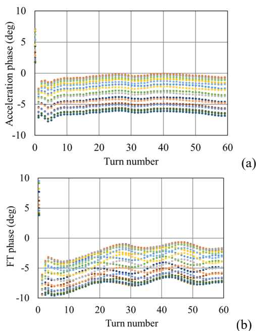
Figure 10: (a) Acceleration and (b) FT phases of 18 particles on the ellipse of 4 \pi \text{mrad} . The acceleration phase means the average of the phases when a particle passes the centerlines of two Dees, and the FT phase that when a particle passes the centerline of the FT Dee.
