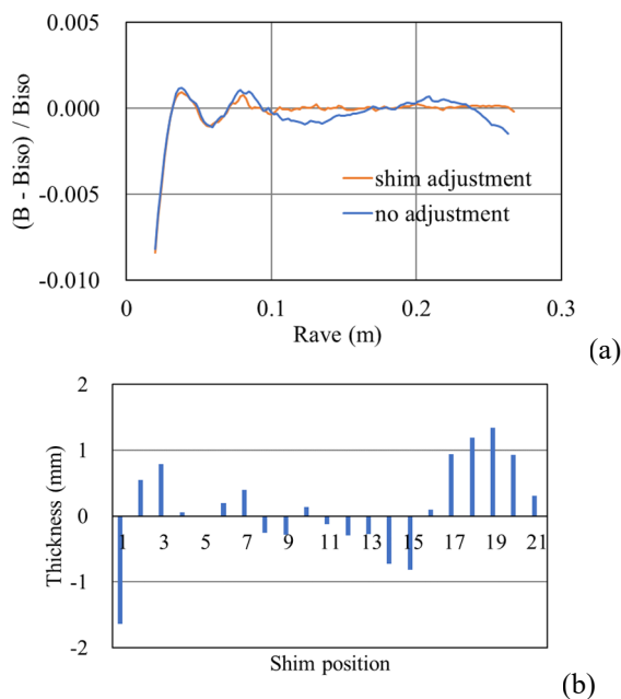
Figure 7: (a) Deviation from the isochronous magnetic field before and after shim correction and (b) adjustment thickness of shims in each position.
