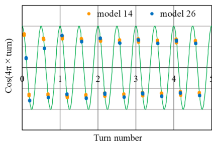
Figure 3: RF phases at passage on the center line of the acceleration gaps.
