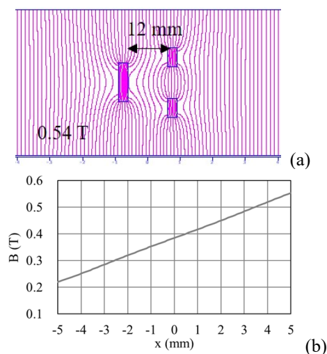
Figure 12: Geometry of iron in the central region of the magnetic channel and (b) magnetic field distribution in the radial direction.
