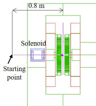
Figure 8: Starting point in the tracking calculations.
