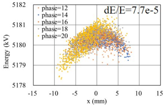
Figure 14: Energies of particles at the exit port. Phase = 12^\circ – 20^\circ means the relative initial phases and absolute is trivial.
