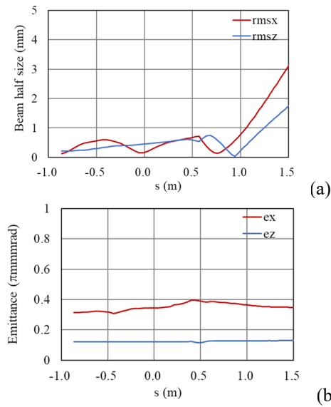
Figure 13: (a) Beam envelopes and (b) emittances in the radial (x) and axial (z) directions in the extraction region. The origin of abscissa s corresponds to the entrance of the deflector.
