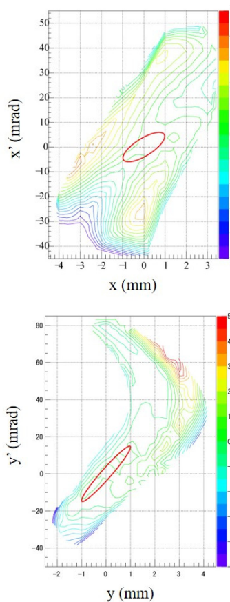
Figure 9: Acceleration acceptance at the starting point in the horizontal (x) and vertical (y) directions. The red ellipses are beam geometry used in the tracking calculations.
