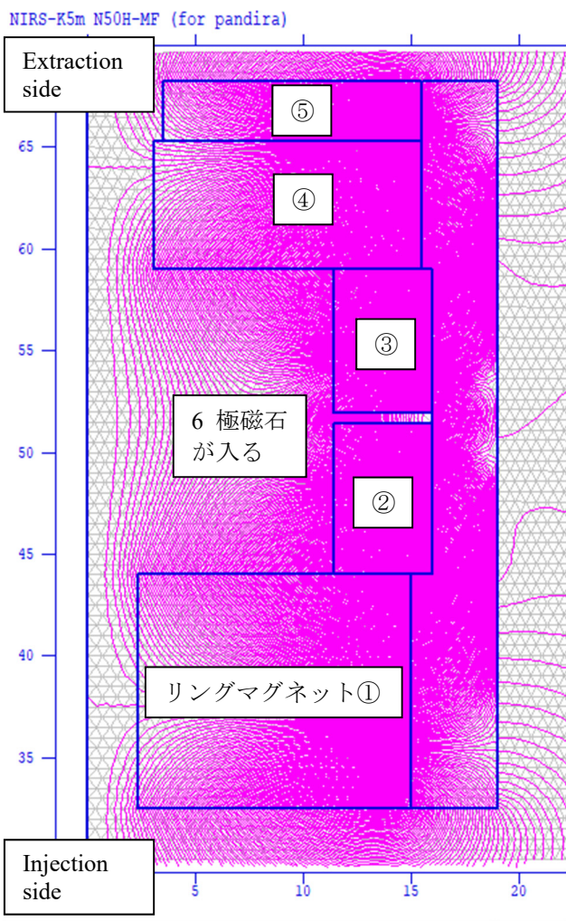
Figure 1: Structure of the ring magnets with iron yoke.
