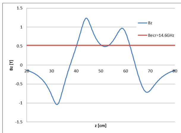
Figure 2: Result of calculation for the mirror magnetic field on the axis made by the ring magnets.
