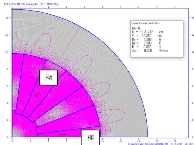
Figure 3: structure of the hexapole magnet.
