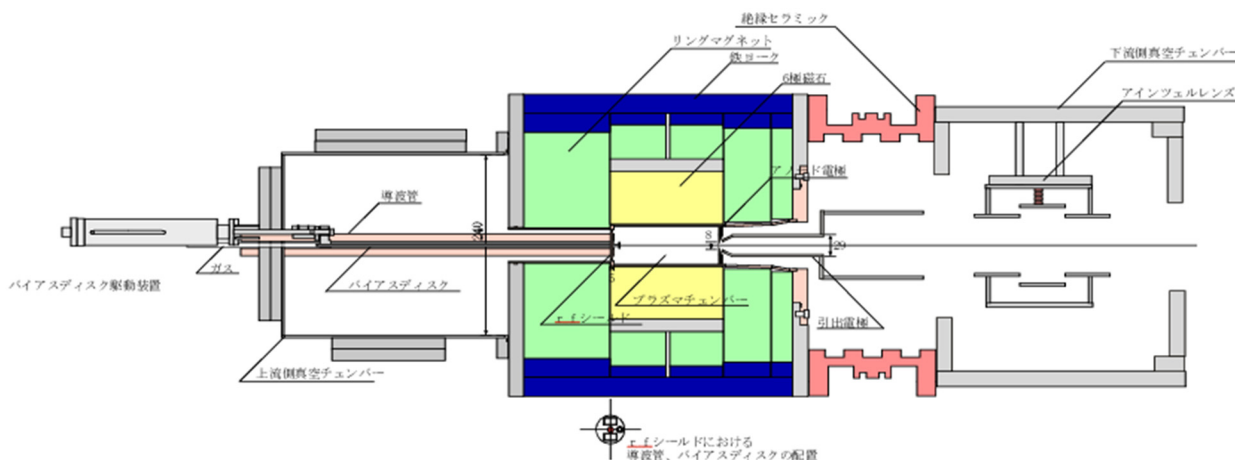
Figure 5: Schematic drawing of new compact ECR ion source with additional waveguide.
