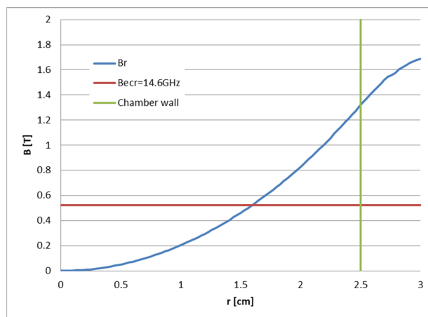
Figure 4: Result of calculation for the hexapole magnet. Blue line is magnetic field. Green line is the chamber wall ( r=25\text{ mm} ). Red line is B_{ocr}=0.521\text{ T} for 14.6 GHz.
