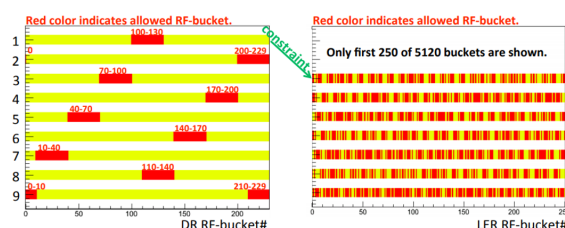
Figure 6: If DR bucket number 0 and 49 are already occupied, only bucket 100 to 130 are available for the new bunches. This constraint also decrease the available buckets at LER.
