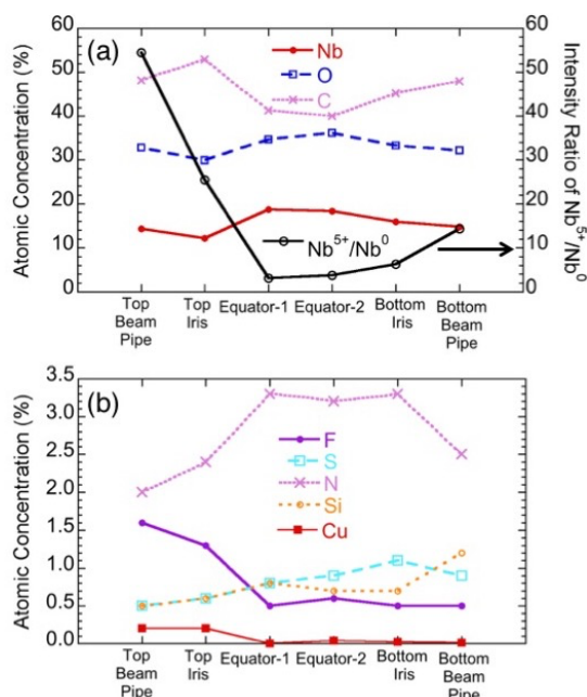
Figure 3: (a) Peak intensity ratios of Nb^{5+} to Nb^0 for all the coupon surfaces. Atomic composition of (a) Nb, O, and C and (b) F, S, N, Si, and Cu elements present on the top surfaces of the electropolished coupons.
