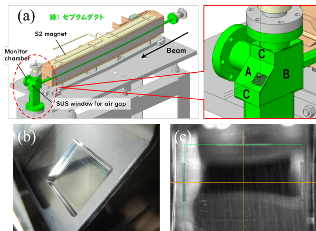
Figure 6: (a) Schematic view of the monitor chamber. Metal window seen from (b) atmosphere side and from (c) vacuum side of the remanufactured septum duct.
