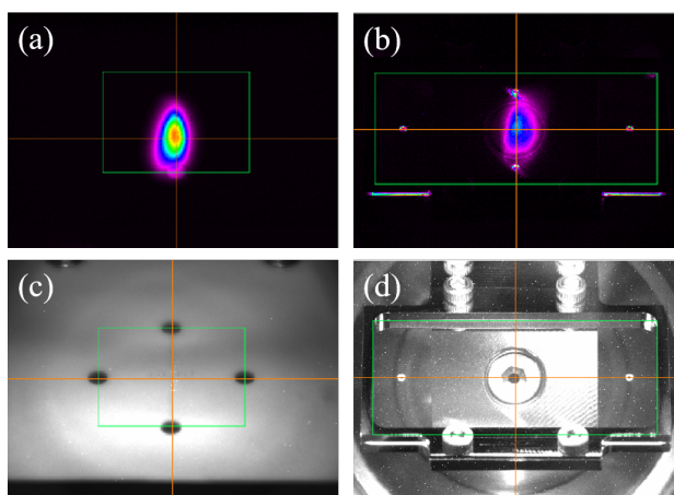
Figure 5: Examples of injection beam profiles obtained with the PM3 (a) before and (b) after the scintillator replacement. Scintillator images taken with the LED light on (c) before and (d) after the replacement.
