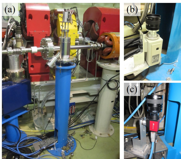
Figure 2: Photos of (a) the PF-BT typical screen monitor and its camera (b) before and (c) after the replacement.
