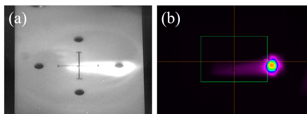
Figure 3: Examples of injection beam profiles obtained with the PM2 (a) before and (b) after the camera replacement. The green frame shown in the right figure is set so as to pass through the centers of the four holes on the fluorescent plates provided as markers.
