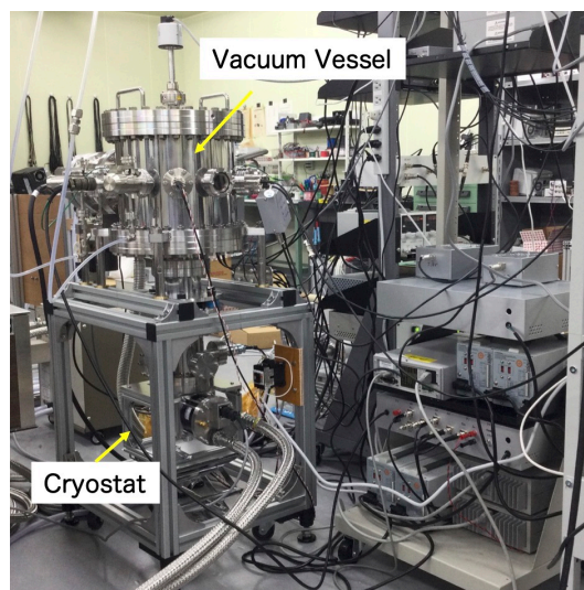
Figure 1: An exterior of new S-POD with the cryogenic buffer-gas cooler.
