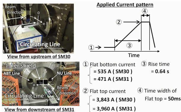
Figure 3: Photographs of SM30 and SM31 (left), and the applied current pattern (right).
