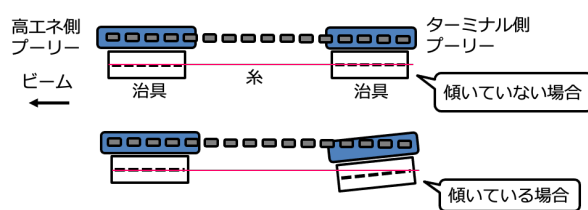
Figure 8: Conducting inclination measurements of the charging chains for the 6 MV tandem accelerator.
