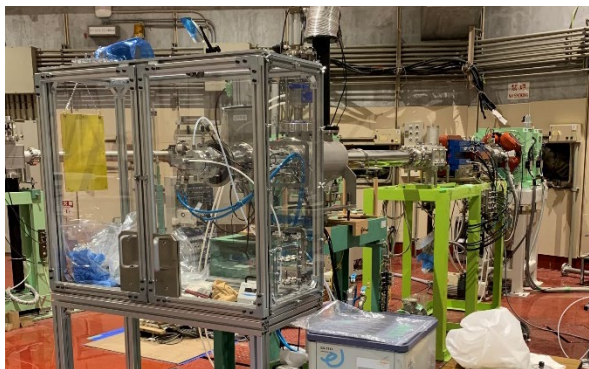
Figure 1: New target system for ^{211}\text{At} production. The blue colored magnets are for beam scanning.
