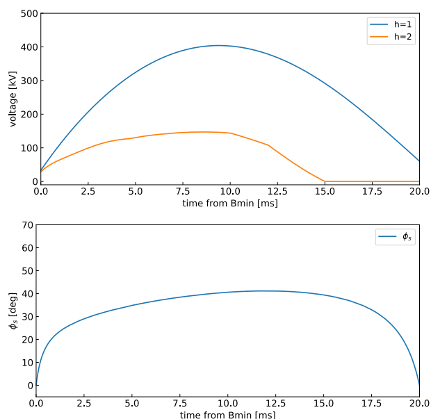
Figure 4: (Top) dual harmonic voltage pattern for initial beam emittance of 10 eVs and (bottom) synchronous phase.
