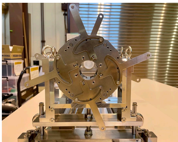
Figure 4: Fabricated prototype magnet.
