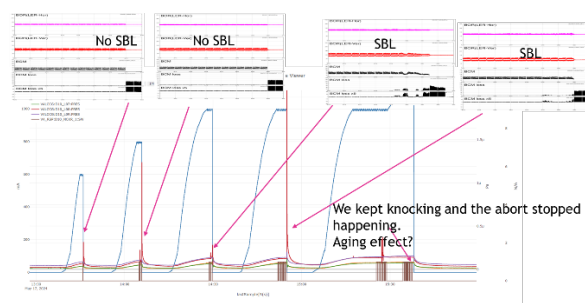
Figure 8: Relationship between knock timing, beam current, and vacuum pressure when (a) a beampipe with a groove and (b) a beampipe with a clearing electrode is knocked, and the plots of BOR/BCM at that time.
