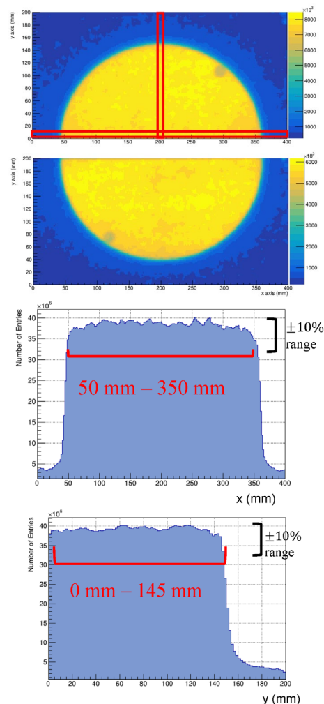
Figure 4: Measured neutron beam profile. Two-dimensional contour (top), horizontal projection (middle), and vertical projection (bottom).
