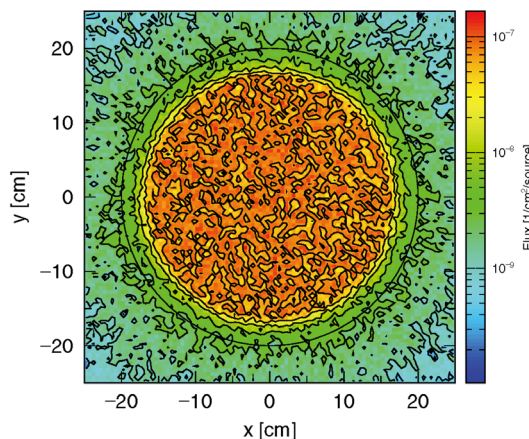
Figure 3: Simulated neutron beam profile.
