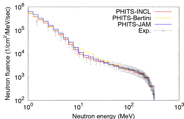
Figure 6: Energy distribution of neutron flux for 1\mu\text{A} proton on target.
