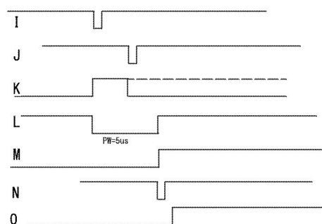
Figure 5: Timing chart of the self-fire/misfire detection circuit.
