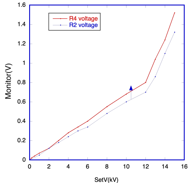
Figure 3: Set voltage versus R4, R2 voltage: The detection voltages are not linear, but the relation between two voltages is same. When the isolation impedance of the thyristor is reduced, the R2 voltage exceeds the R4 voltage.
