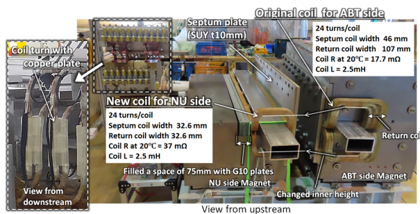
Figure 1: Photograph of new magnetic coil for NU side and original magnetic coil for ABT side.
