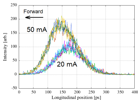
Figure 5: Longitudinal bunch profiles observed at beam currents of 20 mA and 50 mA. For each beam current, five traces were overlaid. Beam energy: 6.5 GeV.
