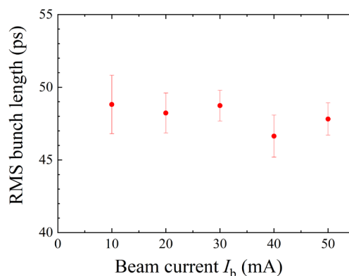
Figure 6: Measured rms bunch length as a function of the beam current. Beam energy: 6.5 GeV.
