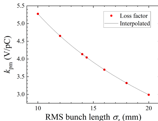
Figure 10: Calculated parasitic-mode loss factor of the APS cavity as a function of the rms bunch length. Solid line indicates a result of interpolation.
