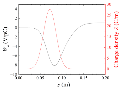
Figure 9: Calculated longitudinal wake potential (black line) of the APS cavity for a bunch length of 14.4 mm. Assumed charge distribution is also indicated by red line.
