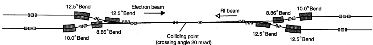
Fig. 5 Side view of the colliding section.
