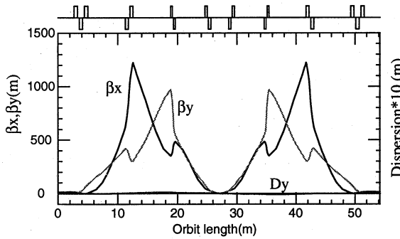
Fig. 7 \beta and dispersion functions in the colliding section of the ion ring.
