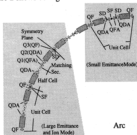
Fig. 2 Composition of the arc section.
