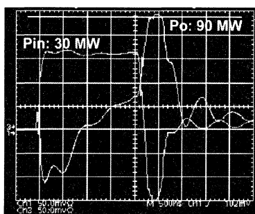
Figure 7: Typical pulse compressor cavity rf power waveforms.
