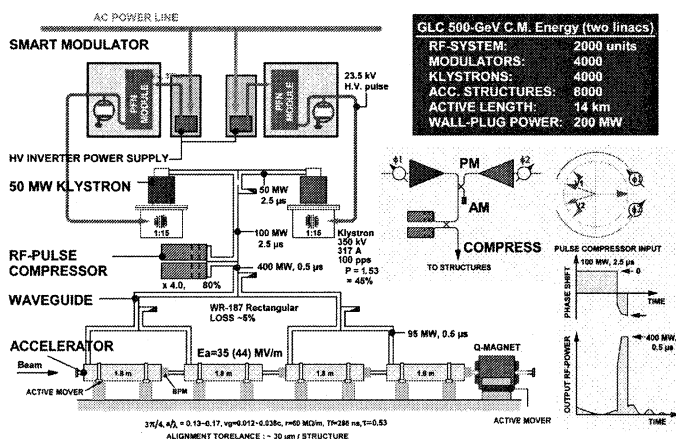
Figure 2: One unit of the C-band main linac.
