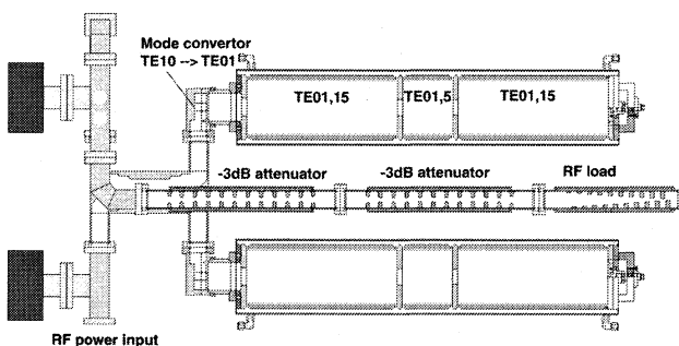
Figure 6: High power test stand for rf pulse compressor cavity.
