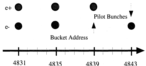
Figure 1: Configuration of bunches at the tail of a train.
