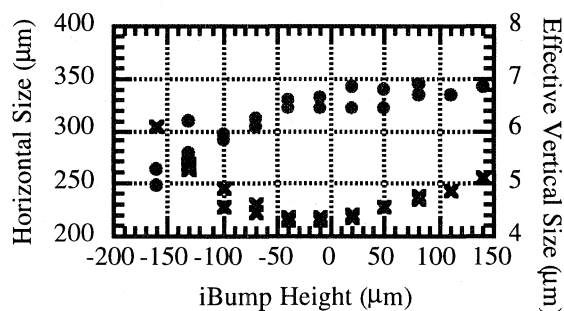
Figure 5: Horizontal size of the electron beam (dots) and the effective vertical beam size (crosses) as a function of the horizontal iBump height. The sizes were not calibrated.
