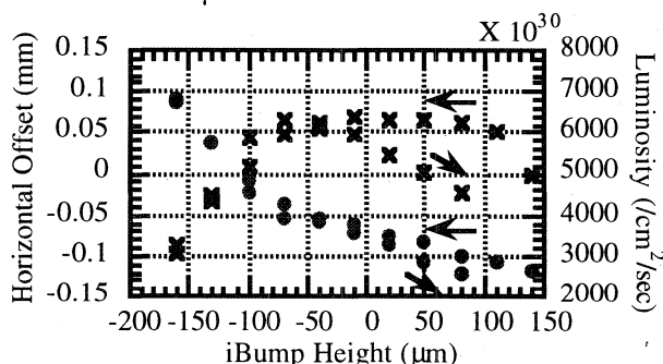
Figure 4: Horizontal position offset (dots) and the luminosity (crosses) as a function of the iBump height, measured with a bunch current of 0.78 mA (LER) and 0.66 mA (HER). The offset data were corrected using values without any collision. The arrows indicate the direction in the iBump height.
