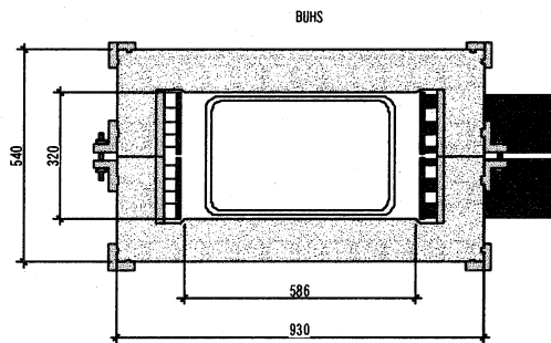
Fig.3 A cross-sectional view of the main bump magnet
