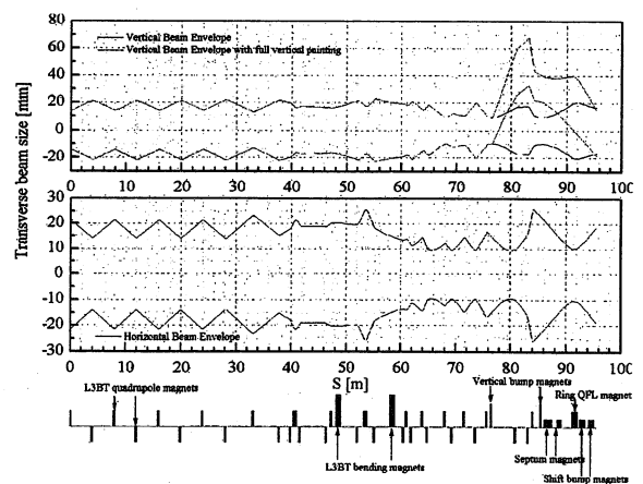
Fig.2 Beam envelope of the injection beam line
