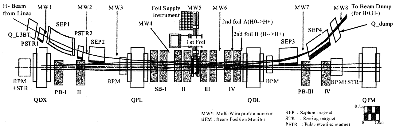
Fig.1 Outline of the H^- injection system
