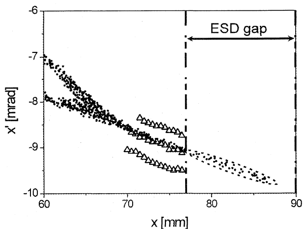
Fig. 1. Triangles represent outgoing separatrix for each momentum of -0.3\% , 0.0\% and 0.3\% from the bottom, as a result of the experiment. Closed circles are simulation result of the separatrix. The area enclosed by dotted line shows extracted beam.
