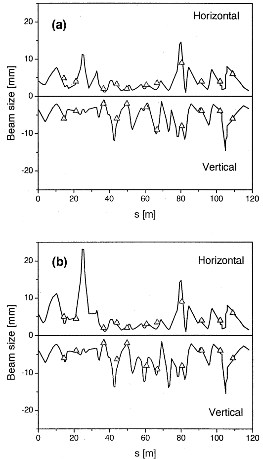
Fig. 3. Comparison of the beam envelope ( 2\sigma ) between the calculation and the measurement (triangles). (a) the momentum spread ( 2\sigma ) is \pm 0.05\% and (b) \pm 0.4\% .
