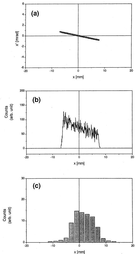
Fig.5. Comparison of the horizontal beam profile between the simulation and the experiment. (a) Estimated phase-space distribution, (b) horizontal profile estimated by the simulation and (c) the measured profile.
