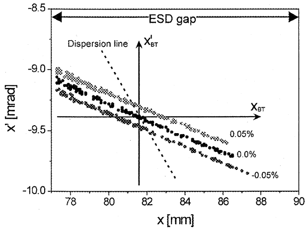
Fig. 2. Simulation result of extracted beam at the entrance of the extraction channel for each momentum of -0.05\% , 0.0\% and 0.05\% from the bottom.
