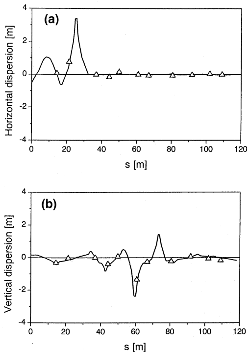
Fig. 4. Comparison of dispersion function between the estimation (line) and measurement (triangles), (a) horizontal and (b) vertical.
