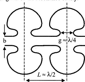
Fig.3. C-band resonance cavity
